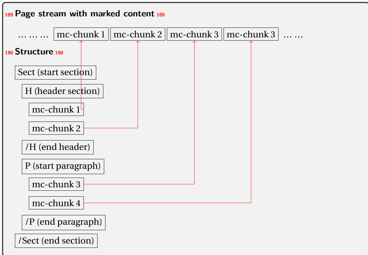
191 Figure 1: Schematical description of the relation between marked content in the page stream and the structure 191
